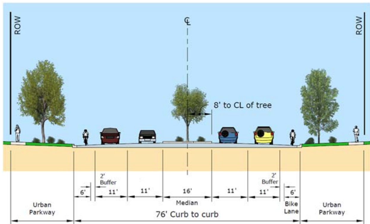
FIGURE 1-30. SECTION A-A: FOUR-LANE MAJOR
